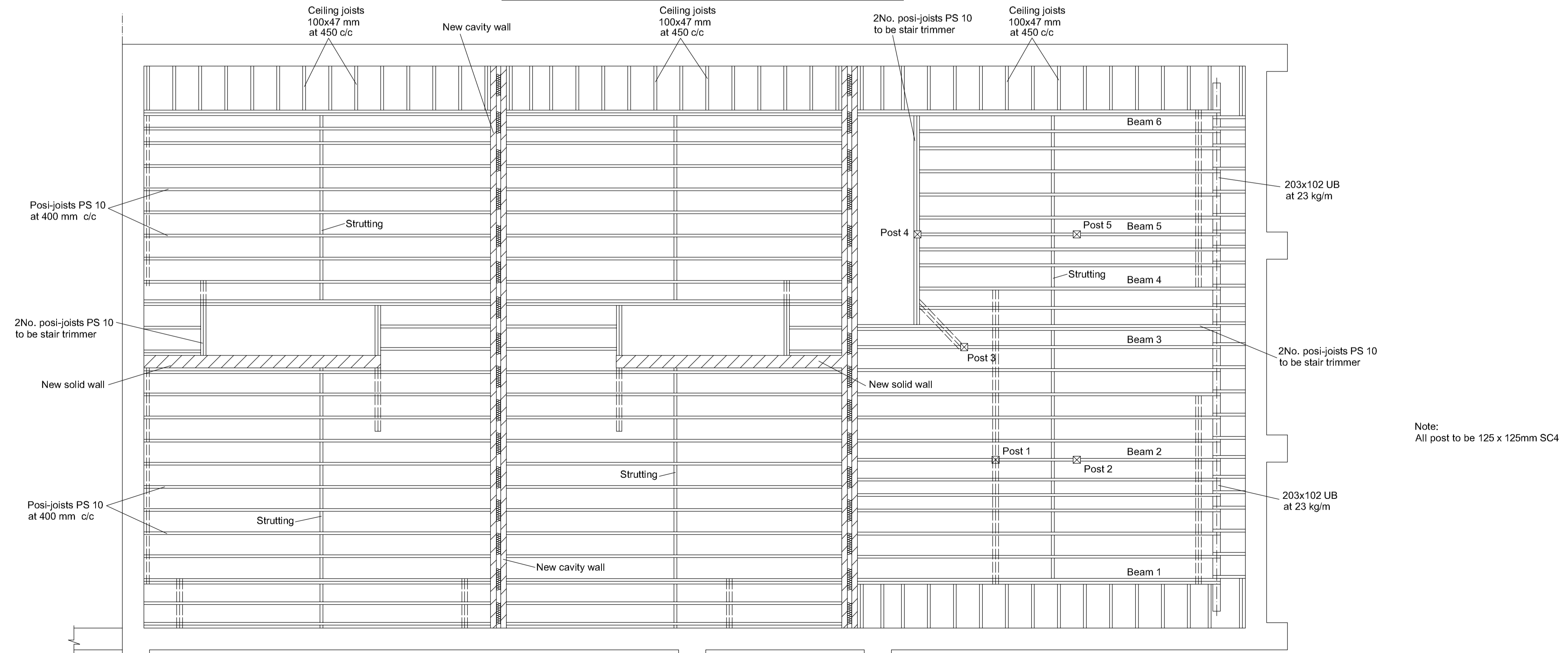
STEELWORK and JOISTS LAYOUT - ATTIC FLOOR
