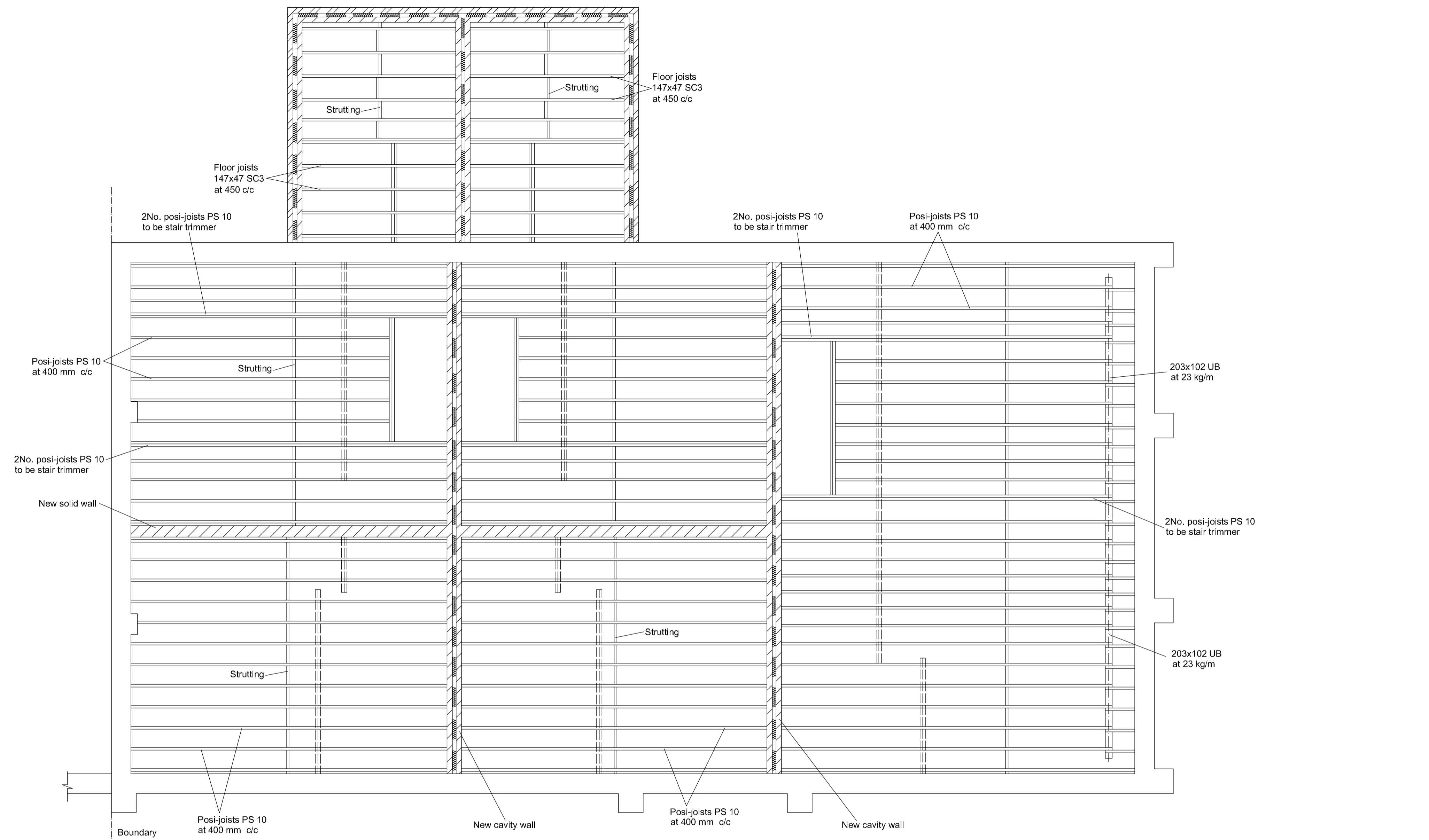
STEELWORK and JOISTS LAYOUT - FIRST FLOOR
